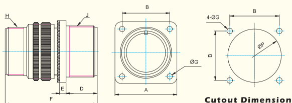
Cutout Dimension
